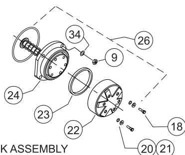
#2 CHECK ASSEMBLY (350 200mm - 300mm) (350A 200mm - 250mm)
