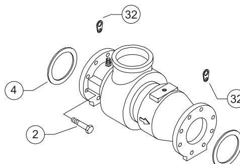
MODEL 350 (100mm - 300mm)
