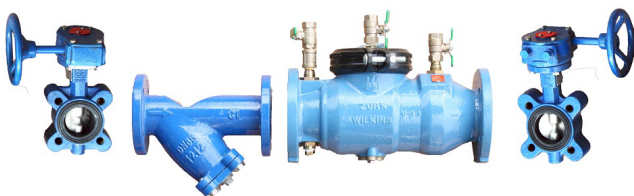
SUFFIX CODE: LCBWO w/ Y-Strainer & Wafer Gear Operated Butterfly Valves
