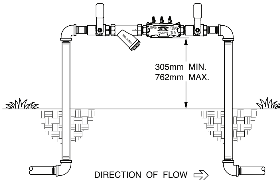
TYPICAL INSTALLATION
